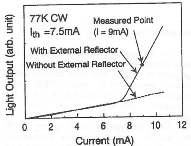
Fig. 4 A current-light output characteristic using external reflector. Lasing operation was obtained only with the external reflector.
