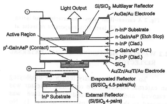
Fig.1 Schematic view of GaInAsP/InP surface emitting laser grown by CBE. For the tuning experiment, evaporated reflector was removed and the external reflector was used.
