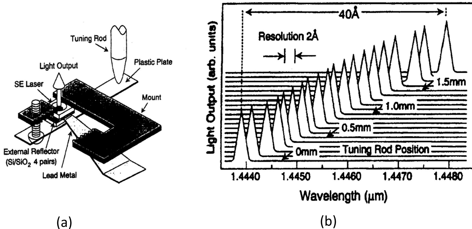
Fig. 7 Continuous-wavelength tuning of an external-cavity surface-emitting laser[A18],[A19]
