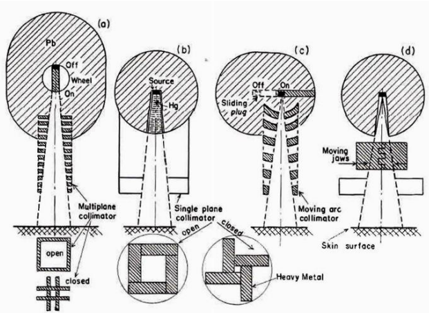
Figure 13. Four types of source shutter arrangements: (a) rotating cylinder with multiplane collimator based on the Johns and Mackay design (b) liquid mercury drawn from a reservoir (not shown), as in Eldorado A design with single plane collimator, (c) sliding drawer design (shown in more detail on the postage stamp of Figure 14) with moving arc collimator, and (d) moving jaw mechanism and single plane collimator. From reference [73]. Courtesy of Charles C Thomas Publisher, Ltd., Springfield, Illinois
