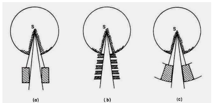
Figure 15. Idealized representation of three common types of diaphragm systems: (a) rectangular blocks, (b) multiple interlocking vanes, and (c) concentric blocks. From [118].
