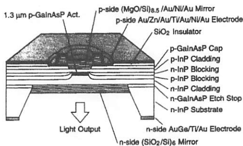
Fig. 1 Structure of GaInAsP/InP surface emitting laser.
