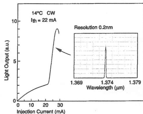
Fig. 2 Room temperature cw lasing characteristic.
