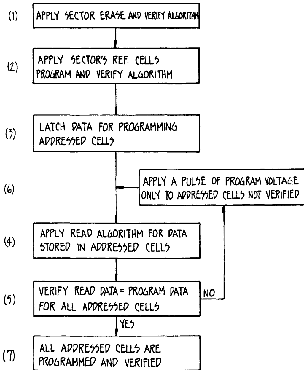
PROGRAM ALGORITHM
