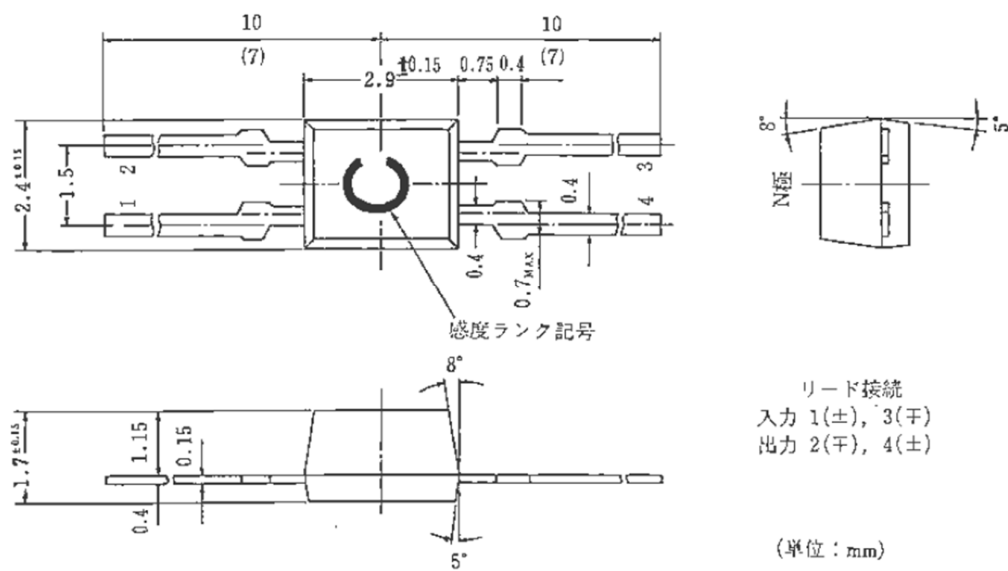
Fig.13 Outline of a high-sensitivity InSb Hall element (HW-300A)
