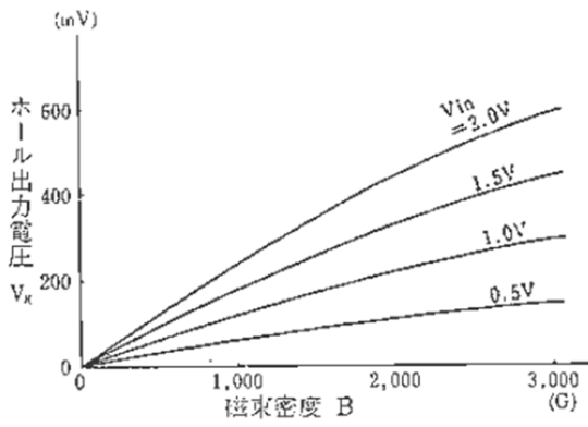
Fig.15 V_H - B characteristics of HW-300C Hall element (constant voltage drive)
