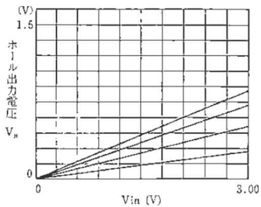
Fig.22 V_H - V_{in} characteristics of HW-300A Hall element
