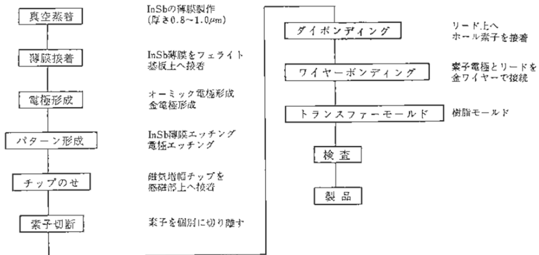
Fig.9 Manufacturing process of high-sensitivity InSb Hall element
