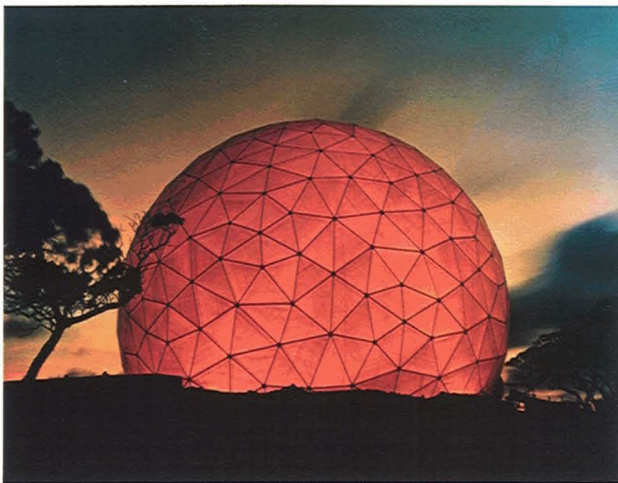
Fig. 12—Photographs of the ALCOR antenna. (a) Interior antenna. (b) Exterior radome.
