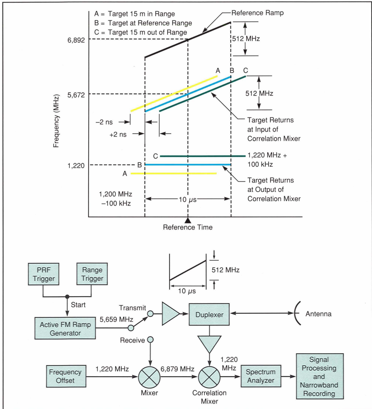
Fig. 15—ALCOR's time-bandwidth exchange.
