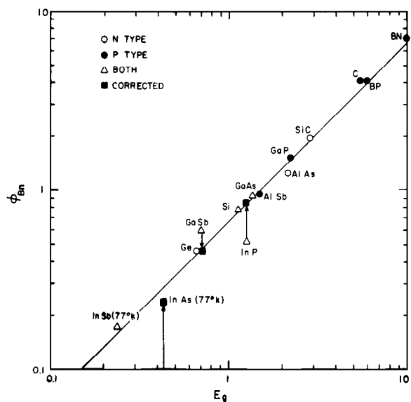
FIG. 3. Barrier energies for zinc-blende materials as a function of the band gap of the semiconductor. See Ref. 14 for the method of obtaining the corrected values.
