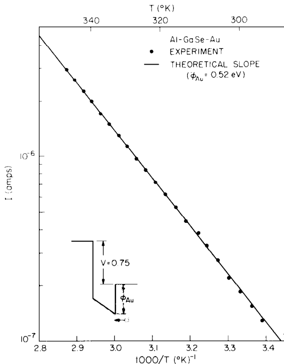
FIG. 7. Current as a function of 1000/T for the Au electrode buried +0.75 V on a 600\text{-}\text{\AA} -thick Al-GaSe-Au structure. The dots are experimental data; the solid line is calculated as described in Ref. 15.
