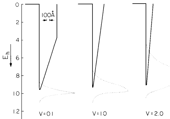
FIG. 6. Theoretical (normalized) current distribution for a reverse biased 600-Å thick Al-GaSe-Au structure. The solid curves illustrate the shape of the image-lowered potential barrier; the dotted curves represent the distribution, as a function of hole energy E_h , of the injected carriers.
