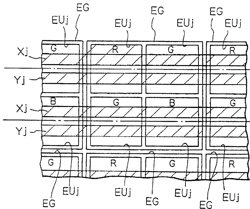
Fig. 6 PRIOR ART
