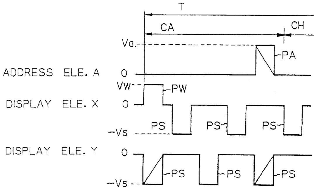
Fig. 5 PRIOR ART
