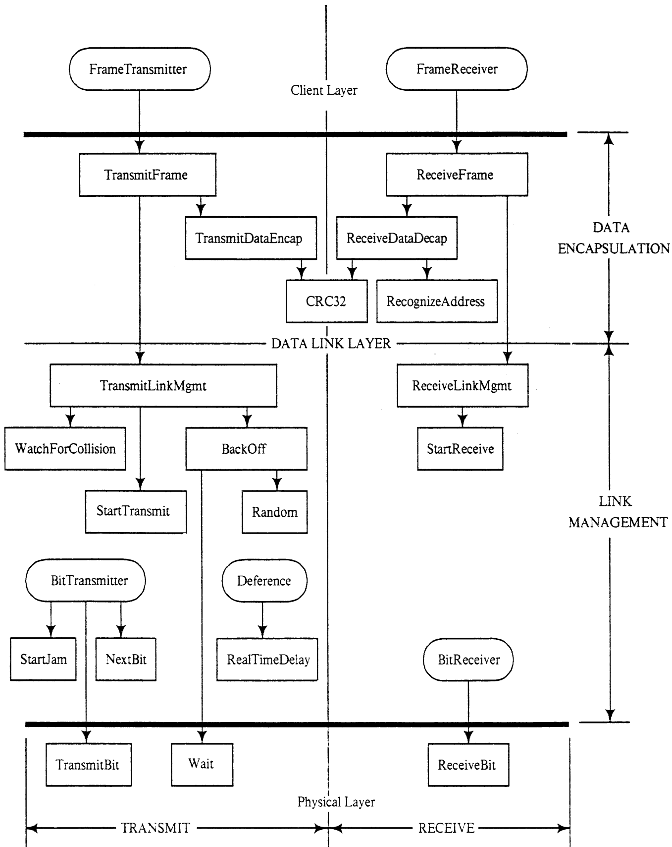
Figure 6-2: Structure of the Data Link Procedural Model
