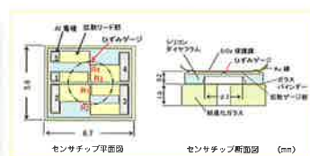
ピエゾ抵抗式半導体圧力センサ Piezoresistive Semiconductor Pressure Sensor
