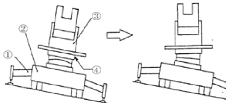
Fig. 2. Inclination compensation for vehicle (1: outrigger, 2: sub-frame, 3: ladder base, 4: upper ring)
