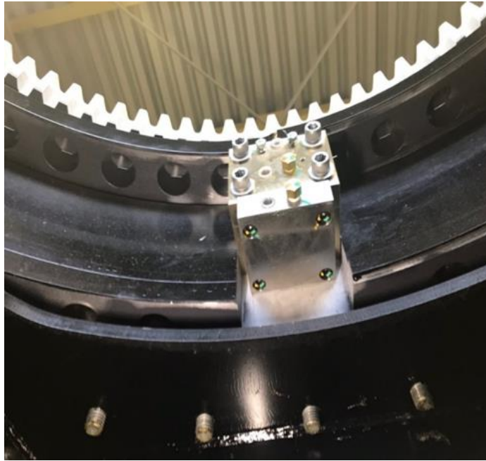
Fig. 3. Lock-cylinder for the lower tilt ring
