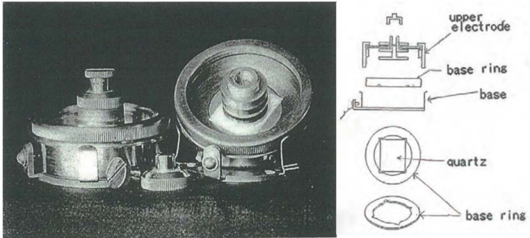
Fig. 4 Koga-type holder used for testing of temperature-insensitive plates (Tokyo Institute of Technology Museum)
