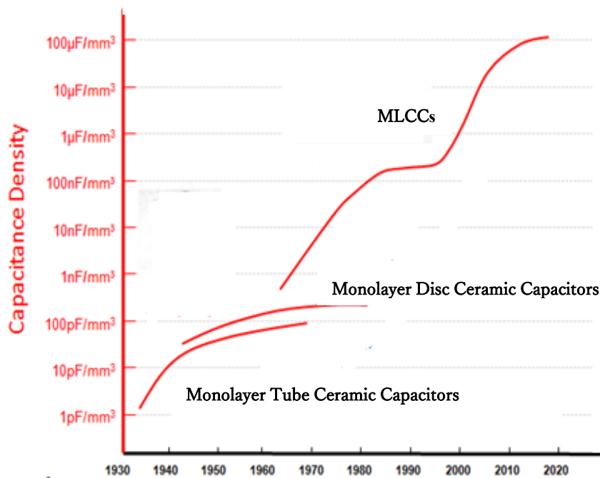
Fig. 1 Changes of capacitance densities of monolayer/multilayer ceramic capacitors
