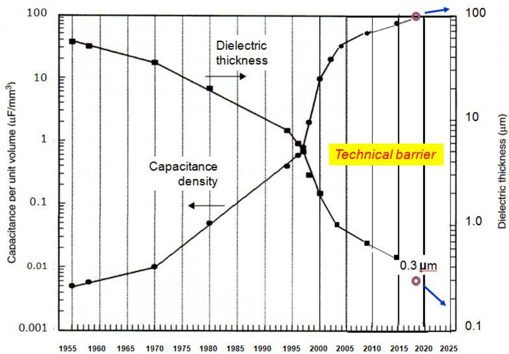
Fig. 2 Changes of capacitance density and dielectric thickness of MLCCs
