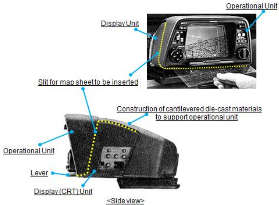
(a) Construction of display equipment to set map sheets
